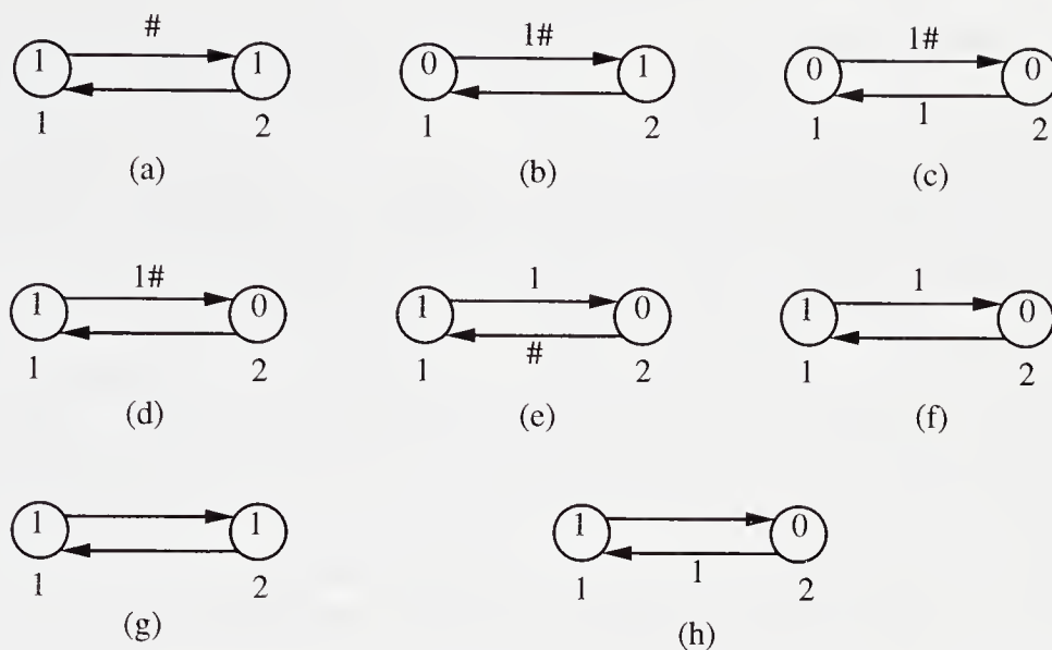
Figure 19.2: Execution of ChandyLamport(A) , for the two-dollar bank.
