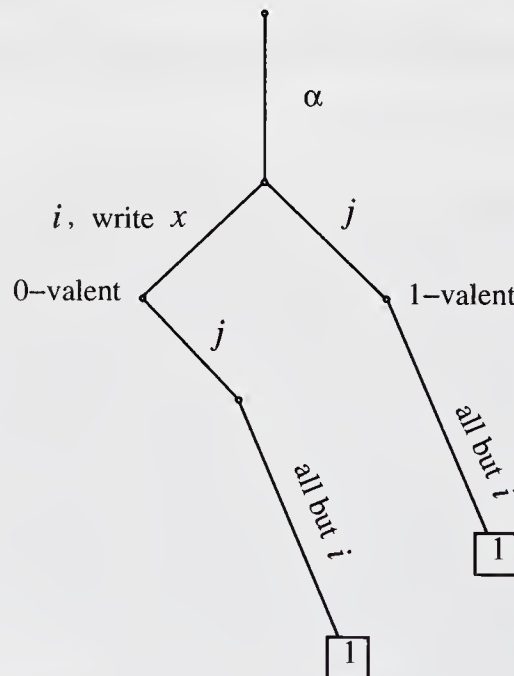
Figure 12.7: Construction for Case 3(b).
