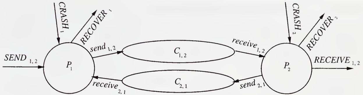
Figure 22.4: External interfaces of processes that crash.
