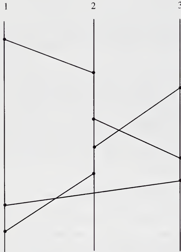
Figure 18.1: Send/receive diagram for execution \alpha .
