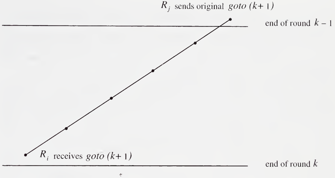
Figure 25.1: goto(k+1) messages relayed from R_j to R_i .
