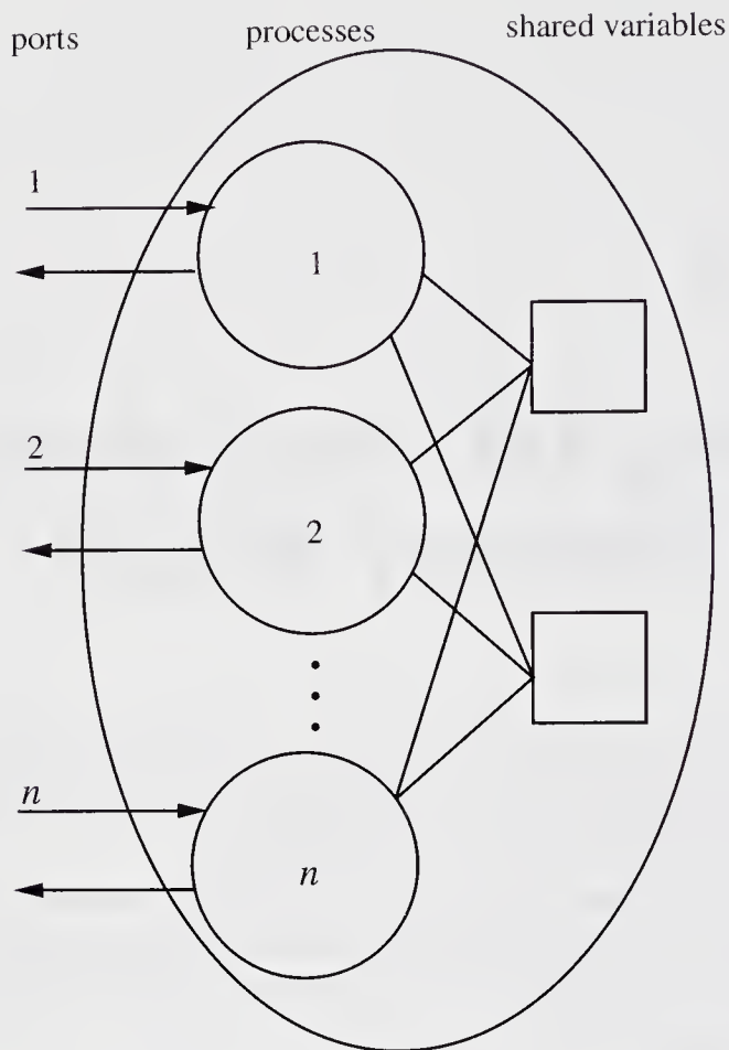
Figure 9.1: An asynchronous shared memory system.
