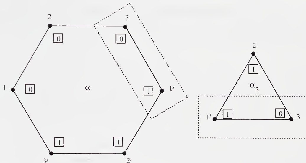
Figure 6.10: Executions \alpha and \alpha_3 are indistinguishable to processes 1 and 3.
