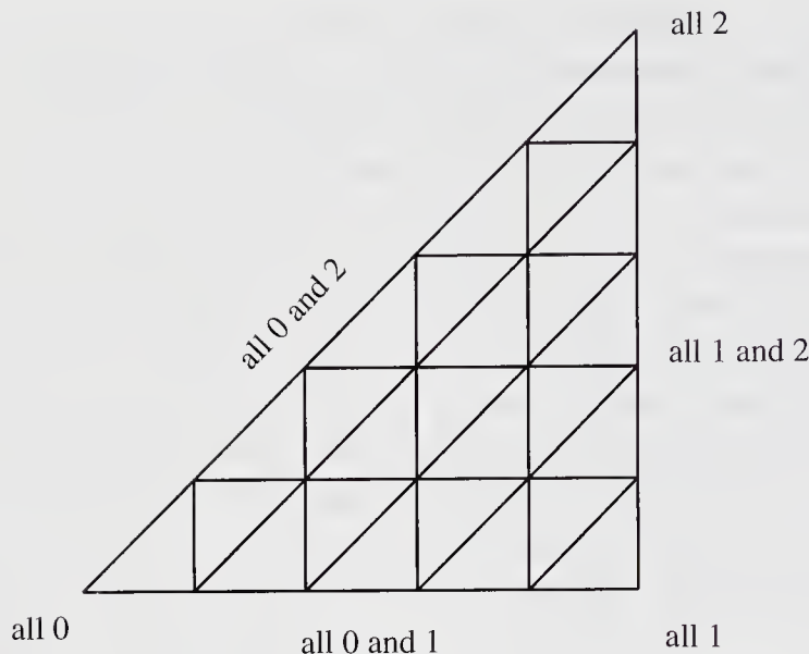
Figure 7.1: Bermuda Triangle for k = 2 .
