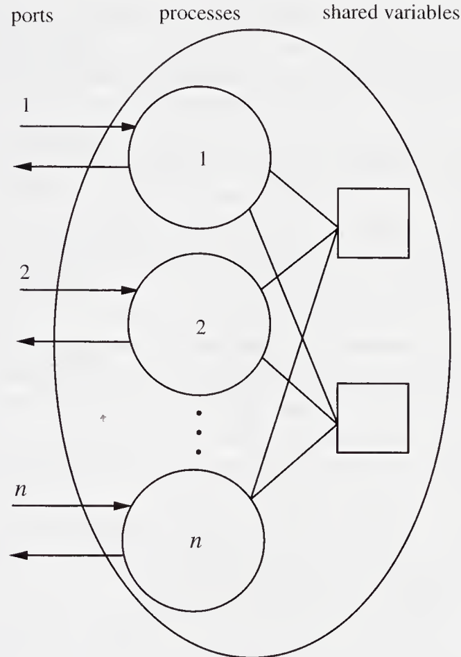
Figure 10.1: An asynchronous shared memory system.
