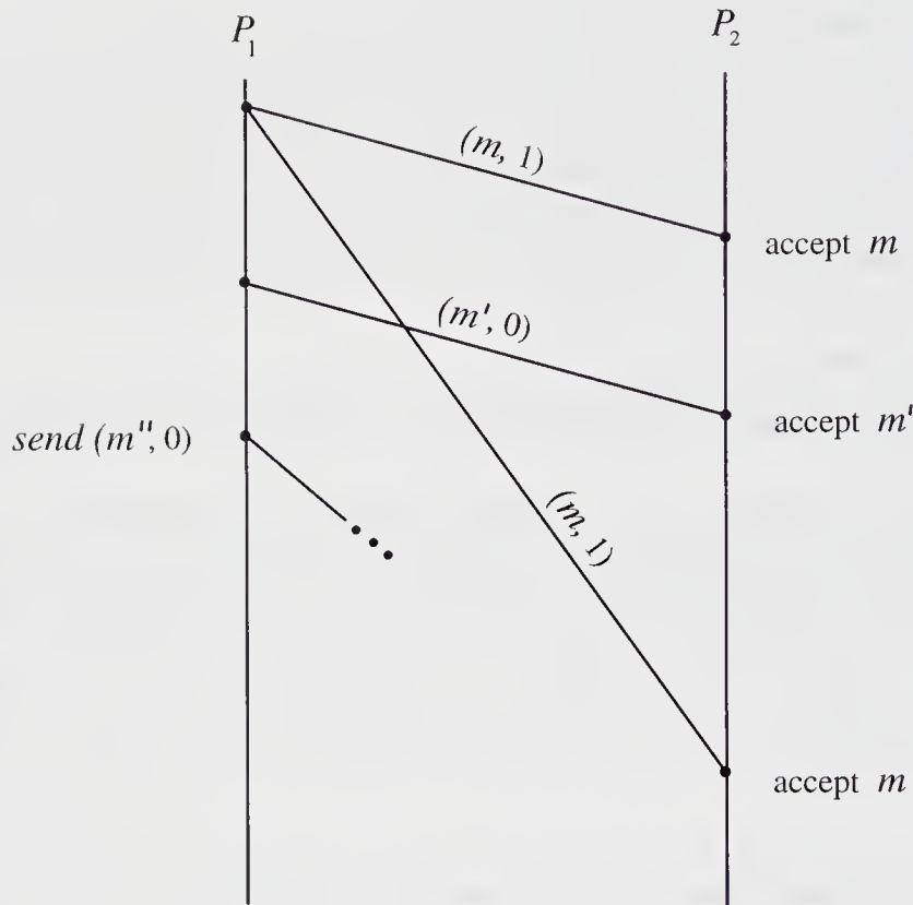
Figure 22.2: P_2 is fooled into accepting m .
