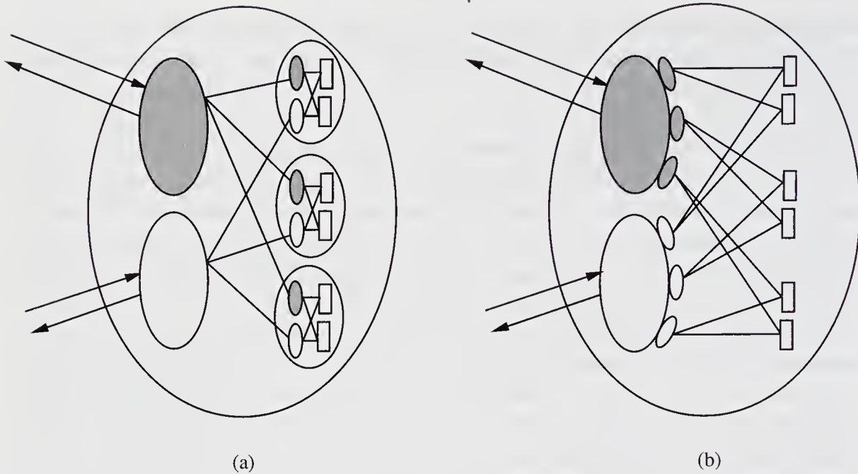
Figure 13.6: Hierarchical construction of a shared memory system.
