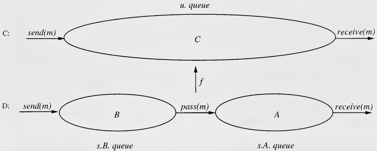
Figure 8.5: Simulation relation f from D to C .
