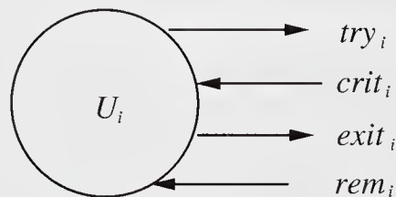
Figure 10.3: External interface of user U_i .
