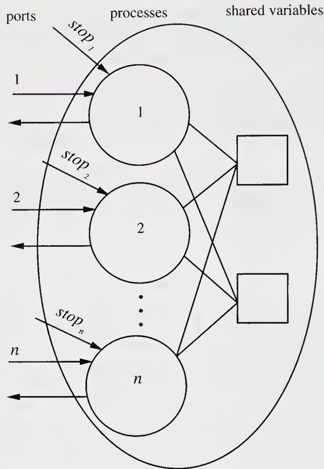
Figure 9.3: Architecture for asynchronous shared memory system with stopping failures.
