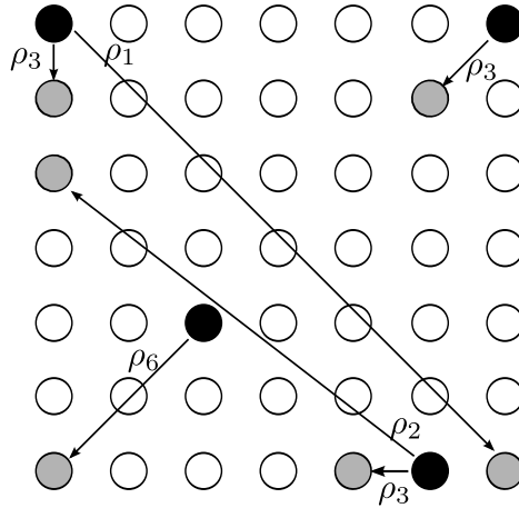
Figure 1.4: Action of the shifts.
