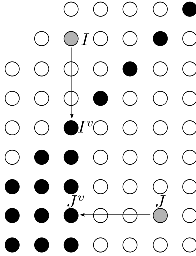
Figure 1.6: Divisorial closure of ideals.
