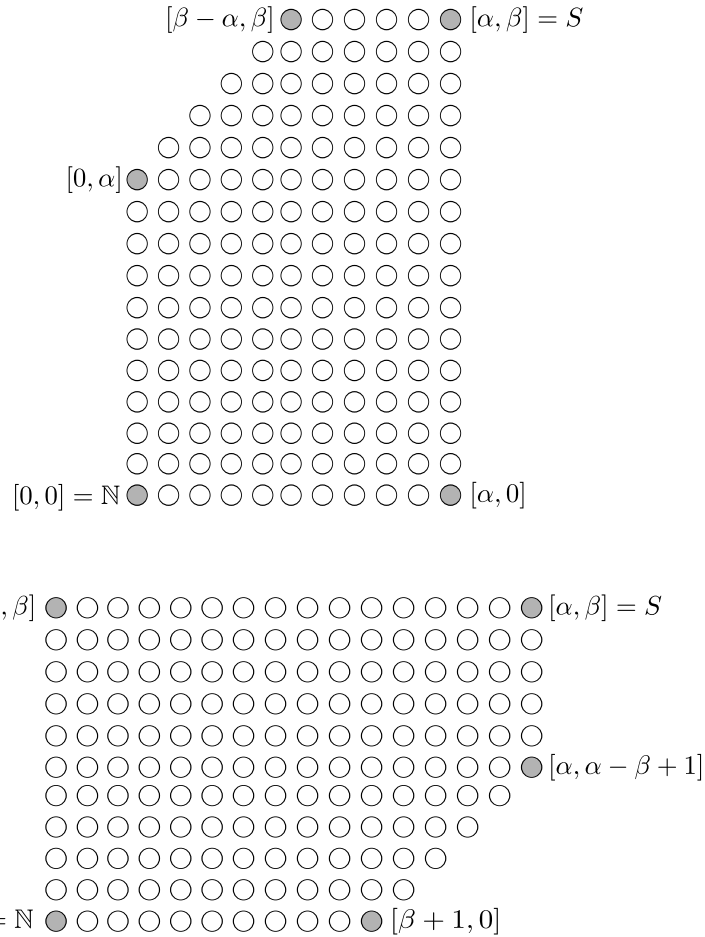
Figure 1.3: Graphical representation of the ideals of a semigroup of multiplicity 3: above, the case \alpha \leq \beta ; below, the case \alpha \geq \beta .
