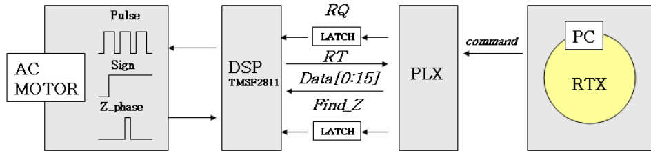
Figure 24. Control system diagram of the sub-controller
