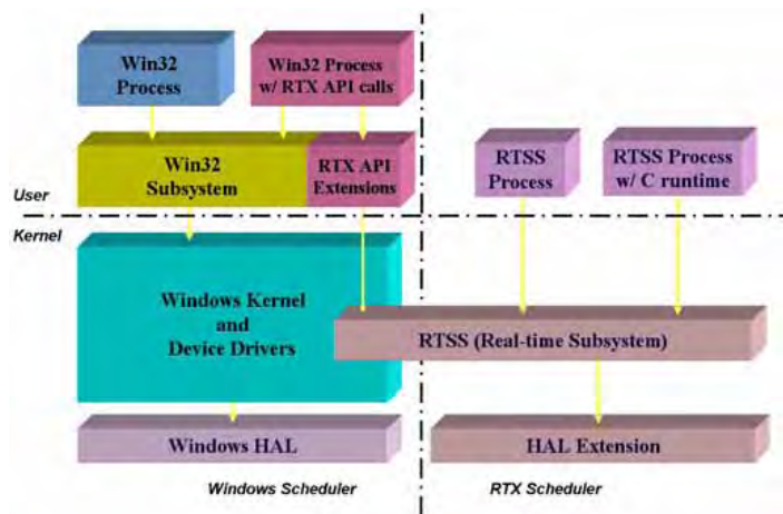
Figure 7. Software Architecture of the OS
