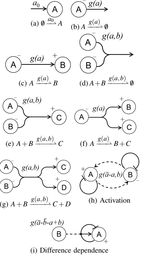
Fig. 1. Graph representations of biochemical reactions.
