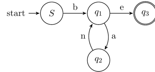
Figure 1: Finite State Automaton, accepting the pattern b(an)^+e
