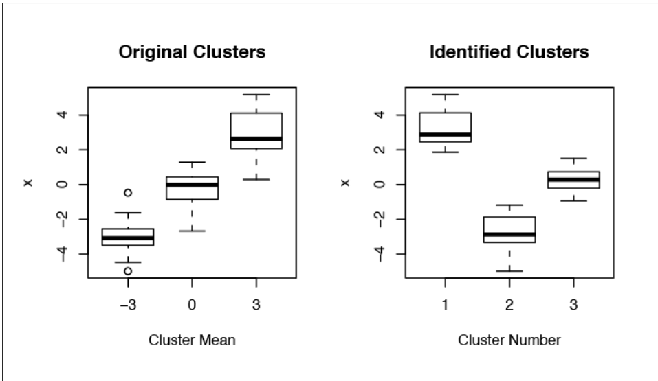
Figure 13-3. Clusters comparison
