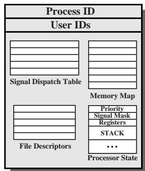
UNIX Process Structure
