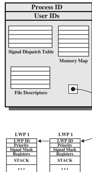
Solaris 2.x Process Structure
