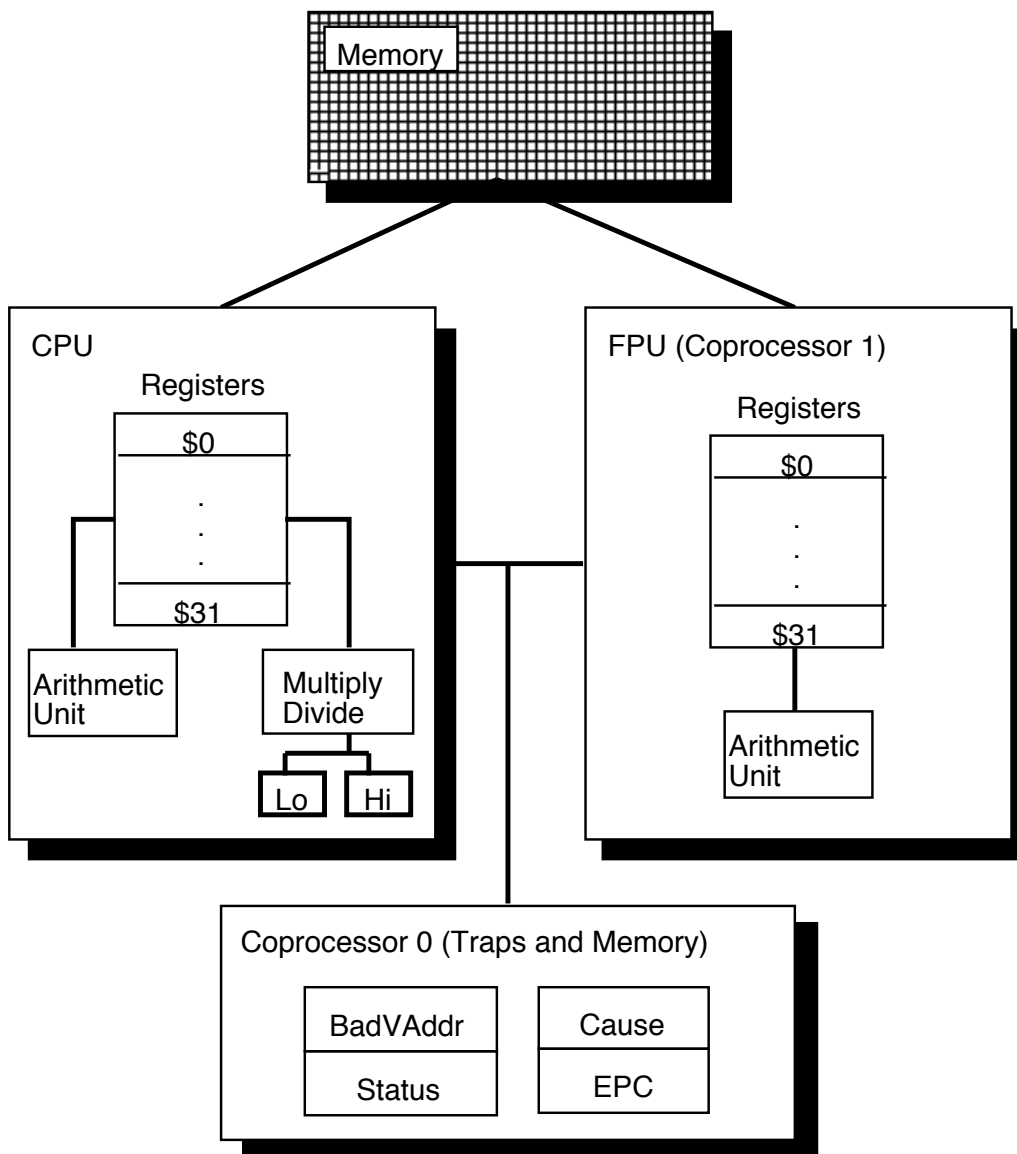
Figure 2: MIPS R2000 CPU and FPU
