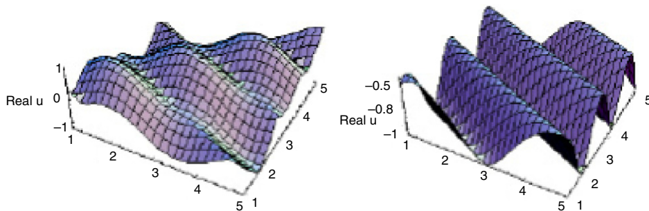
Fig. 3b. The surface shows the real part of solutions (5.43) with \phi(\zeta) = u_1 , w = w_2 , p = 1 , r = -2 , \Omega = -1 , \lambda = 2/3 , k_1 = 1 , k_3 = -2 , P = 1 , Q = -1 , R = 1 , k = -1 , A = -3 , B = -3 , D = 6 , C = 3/2 .
