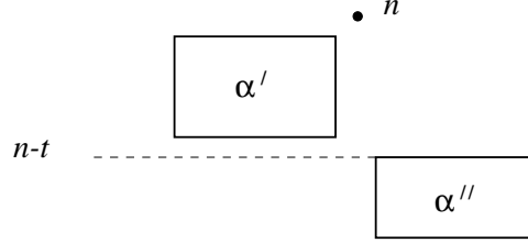
FIGURE 4. The block decomposition for \alpha \in \mathfrak{S}_n(132)
