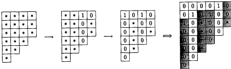
FIG. 4. Manipulations of Lemma 5 in the context of 0-1 tableaux.
