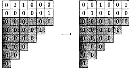
FIG. 5. Bijection between two classes of 0-1 tableaux.
