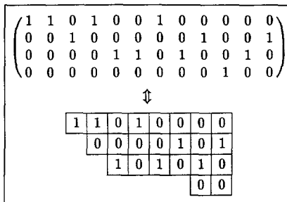
FIG. 1. Correspondence between partitions and 0-1 tableaux.
