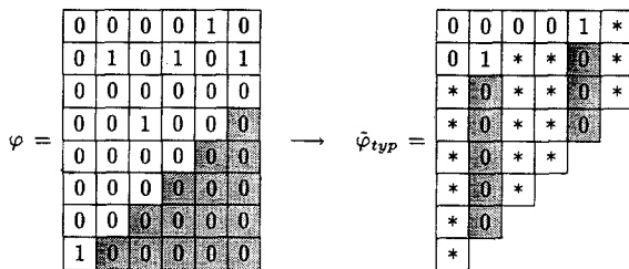
FIG. 3. Encoding of \tilde{w}_b as a 0–1 tableaux.
