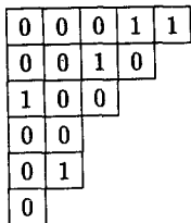
FIG. 2. Correspondence between permutations and 0-1 tableaux.
