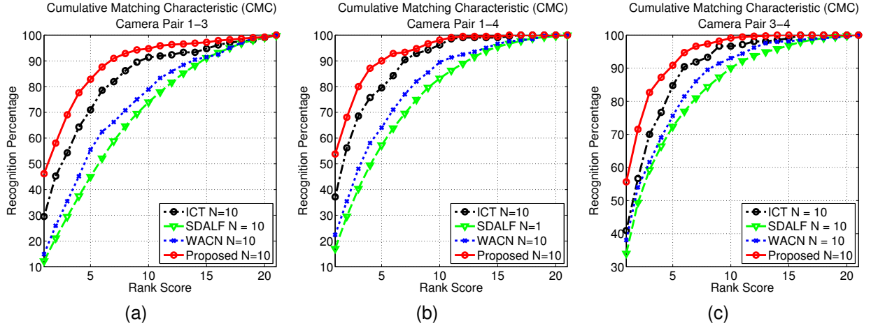
Fig. 10. CMC curves for RAiD dataset. In (a), (b) and (c) comparisons are shown for the camera pairs 1-3, 1-4 and 3-4 respectively.
