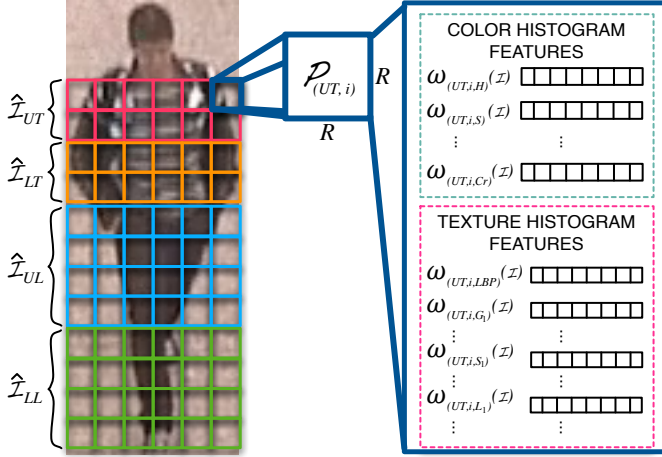
Fig. 6. Dense image features from the detected body parts. Dense color and texture histogram features are extracted from each of the 4 resized body parts.
