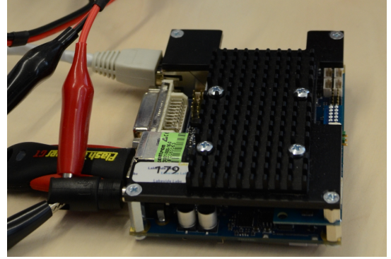
Fig. 12. The pITX-SP hardware platform used in our tests.
