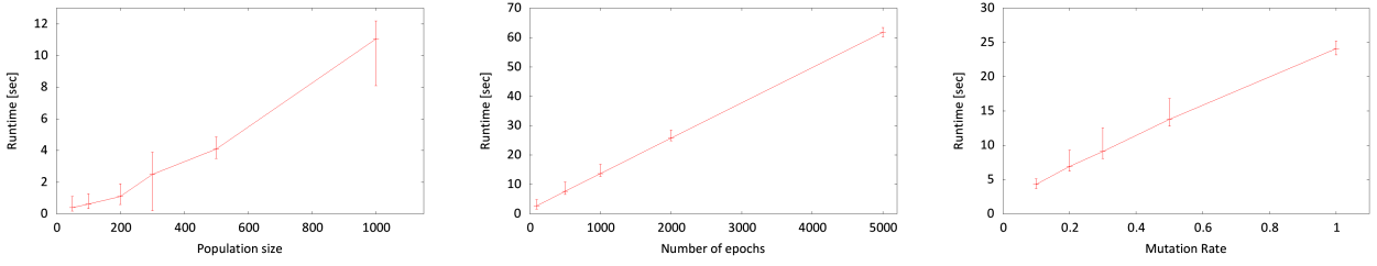
(a) Population size. 1000 epochs. Mutation rate: 0.5. (b) Number of Epochs. Population size: 1000. Mutation rate: 0.5. (c) Mutation Rate. 1000 epochs. Population size: 1000
