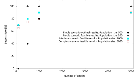
Fig. 6. The relation between number of epochs and the rate of finding optimal and feasible results (success rate), respectively.
