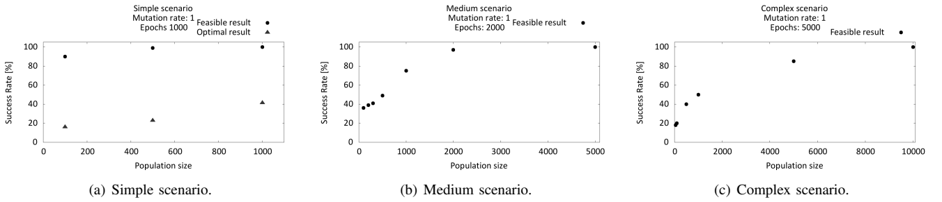
Fig. 7. Relation between population size and the rate of finding feasible results (success rate).
