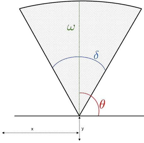
Fig. 2. The 2D model of the camera's field of view which is defined by the covering angle \delta (blue) and the covering distance \omega (green) and the orientation \theta (red). The location of the sensor are depicted by x and y . The field of view is indicated as gray area.
