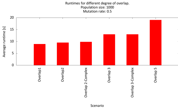
Fig. 10. The runtimes for our overlap scenarios.
