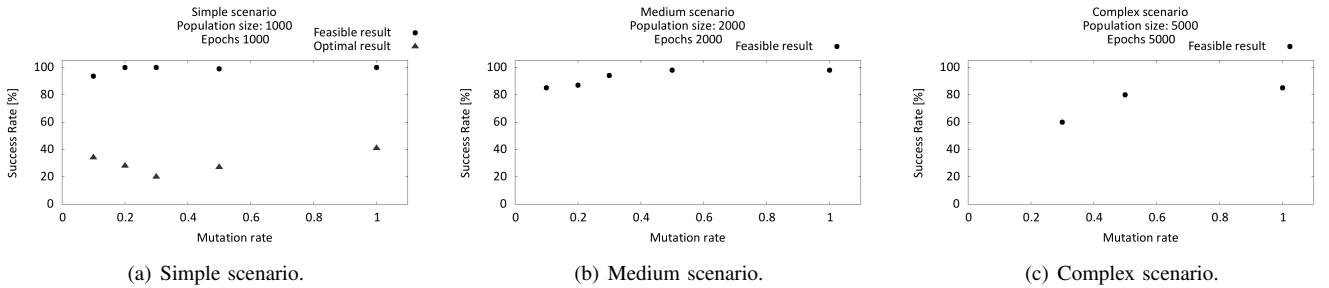
Fig. 8. The relation between mutation rate and the rate of finding feasible results (success rate).
