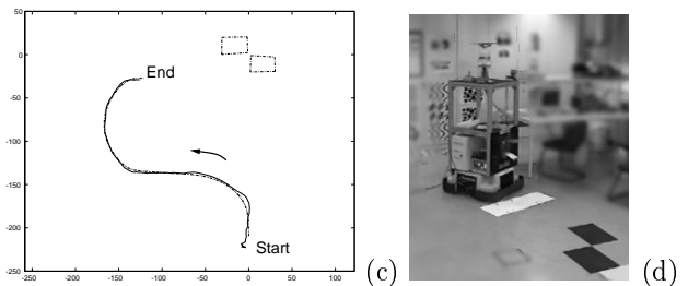
Fig. 14. Visual Path Following, with the trajectory specified in image coordinates. (a) x, y positions before (dotted line) and after filtering (solid line). (b) Orientation before (dotted line) and after filtering (solid line). (c) Dash-dotted line shows the landmark that defines the origin. The dotted line is the specified trajectory and the solid line shows the filtered position estimates. (d) Image of mobile robot at the end of path following.
