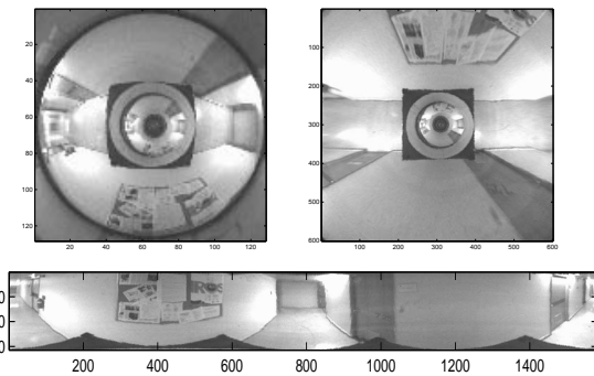
Fig. 4. Top: omni-directional image (left) and corresponding bird's eye view (right). Bottom: panoramic image.
