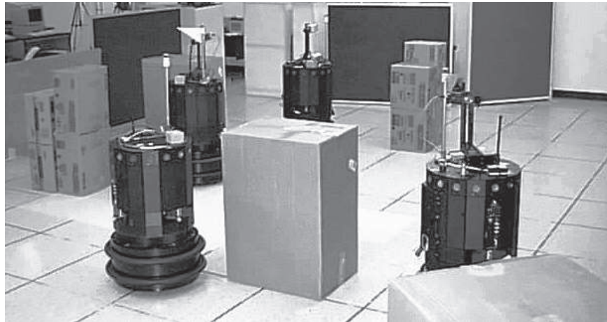
Figure 8.5 Robots cooperatively tracking an object under the ALLIANCE architecture. (Photograph courtesy of Oak Ridge National Laboratories.)
