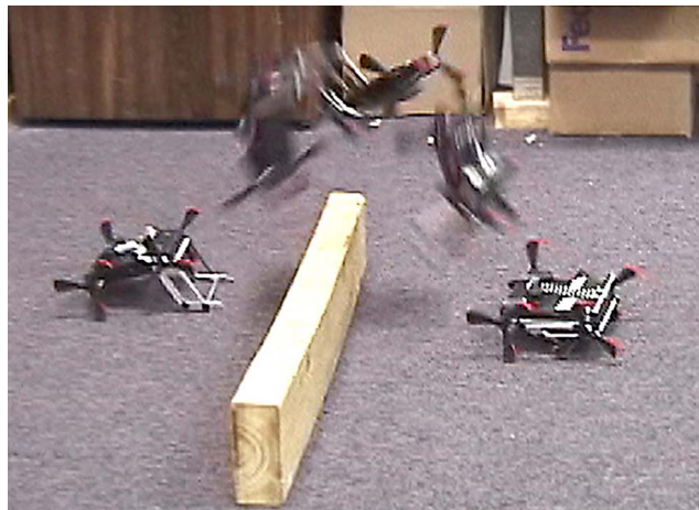
Fig. 6 Composite of video frames showing Mini-Whegs™ 9J jumping high over a 9 cm barrier.
