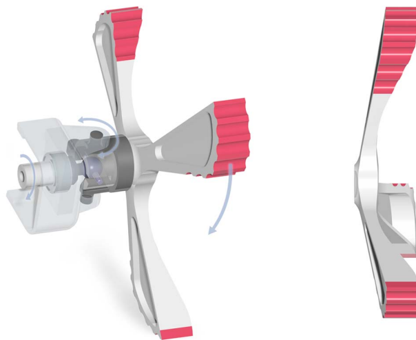
Fig. 4 Renderings of the current Mini-Whlegs™ steering mechanism (left) and the new splayed leg design (right).
