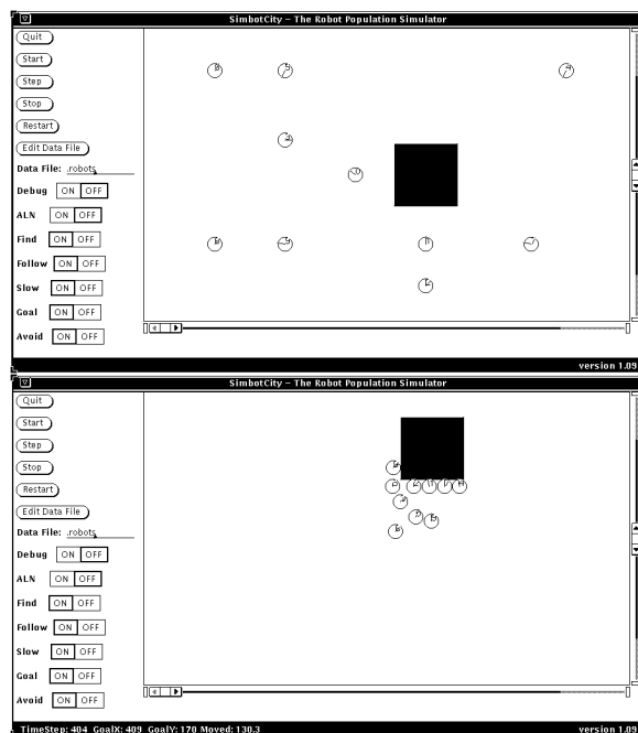
Figure 6: The initial configuration of the cooperative box-pushing task (top) and after 404 simulation steps in which the box has been moved 130 units upwards. The robots (circles) must locate and push the large box, which is too heavy to be moved by a single robot; therefore requiring the cooperative effort of at least 2 robots pushing on the same side.
