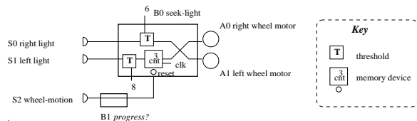
Figure 4: A progress “virtual stimulus-response” behavior monitors wheel-motion and constantly resets an interval counter.
