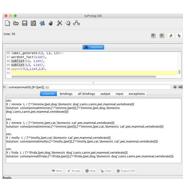
Figure 1: label_generate/3 example: WordNet case study
