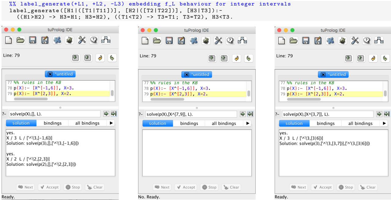
Figure 2: label_generate/3 example: numeric interval intersection
