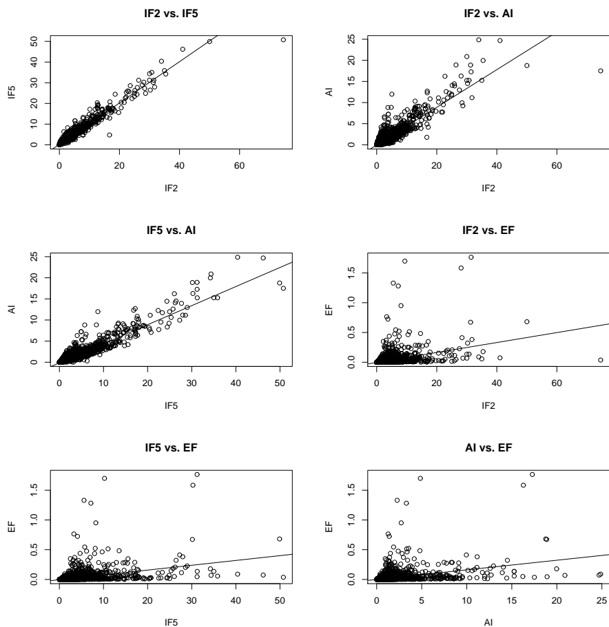
Figure 3: Linear regression models for each pair of indicators.
