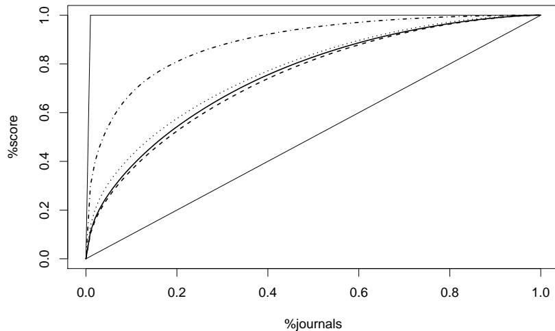
Figure 1: Inverted Lorenz diagram with curves for IF2 (solid), IF5 (dashed), AI (dotted), and EF (dot-dashed). The curves are contained in a triangle representing the extreme cases of equidistribution (the side of the triangle corresponding to the segment with slope 1) and maximum concentration (the other two sides of the triangle).
