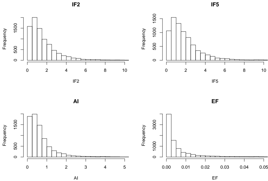
Figure 2: Histograms for factors of journal influence.
