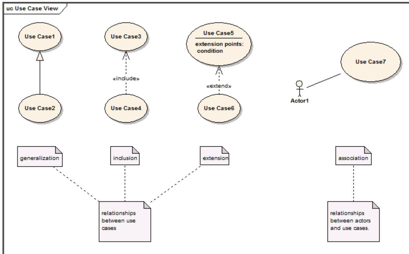
Figure 1 - Use Case notation
