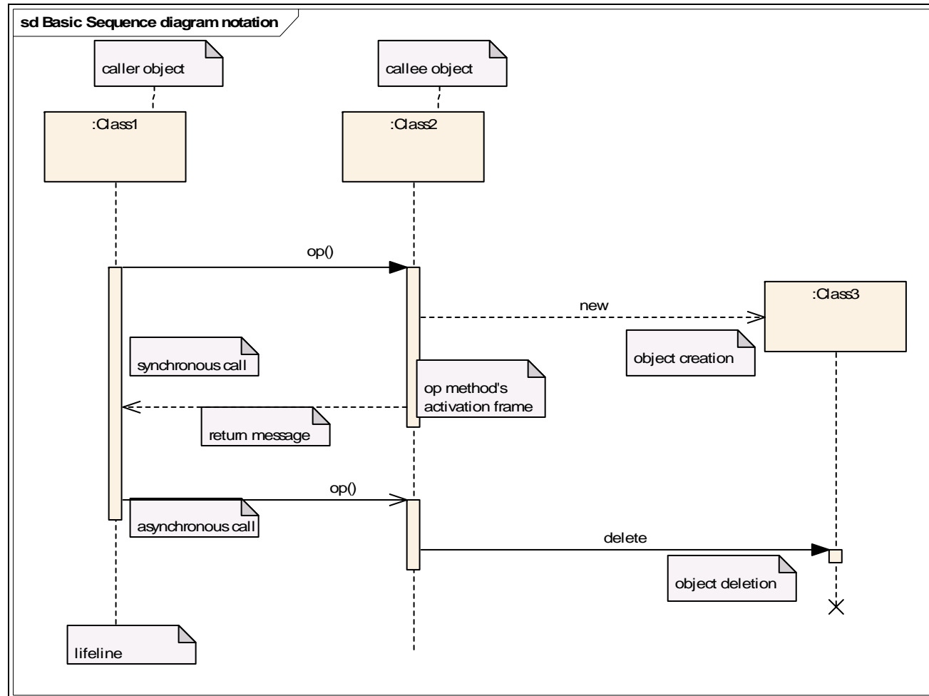
Figure 3 - Sequence diagram notation (Basic)
