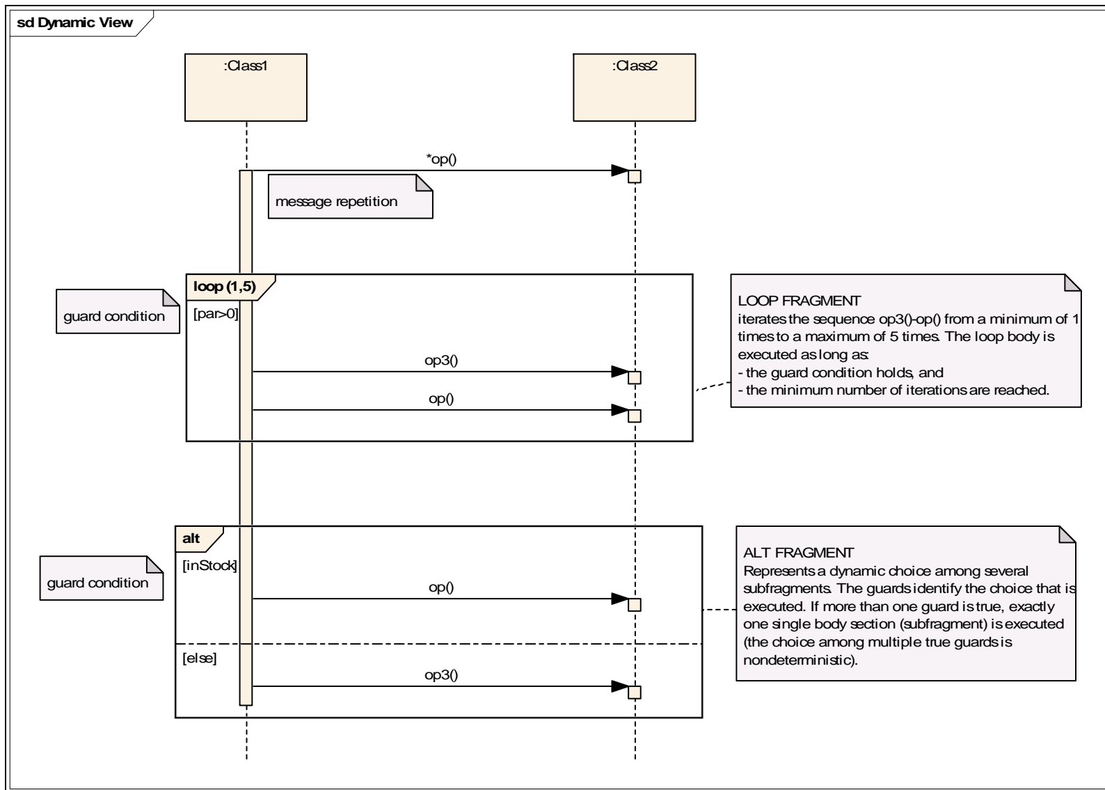
Figure 4 - Sequence Diagram notation - fragments and loops
