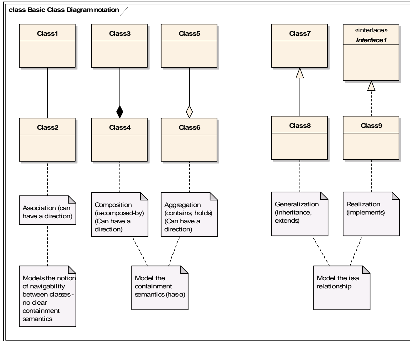
Figure 2 - Class diagram notation
